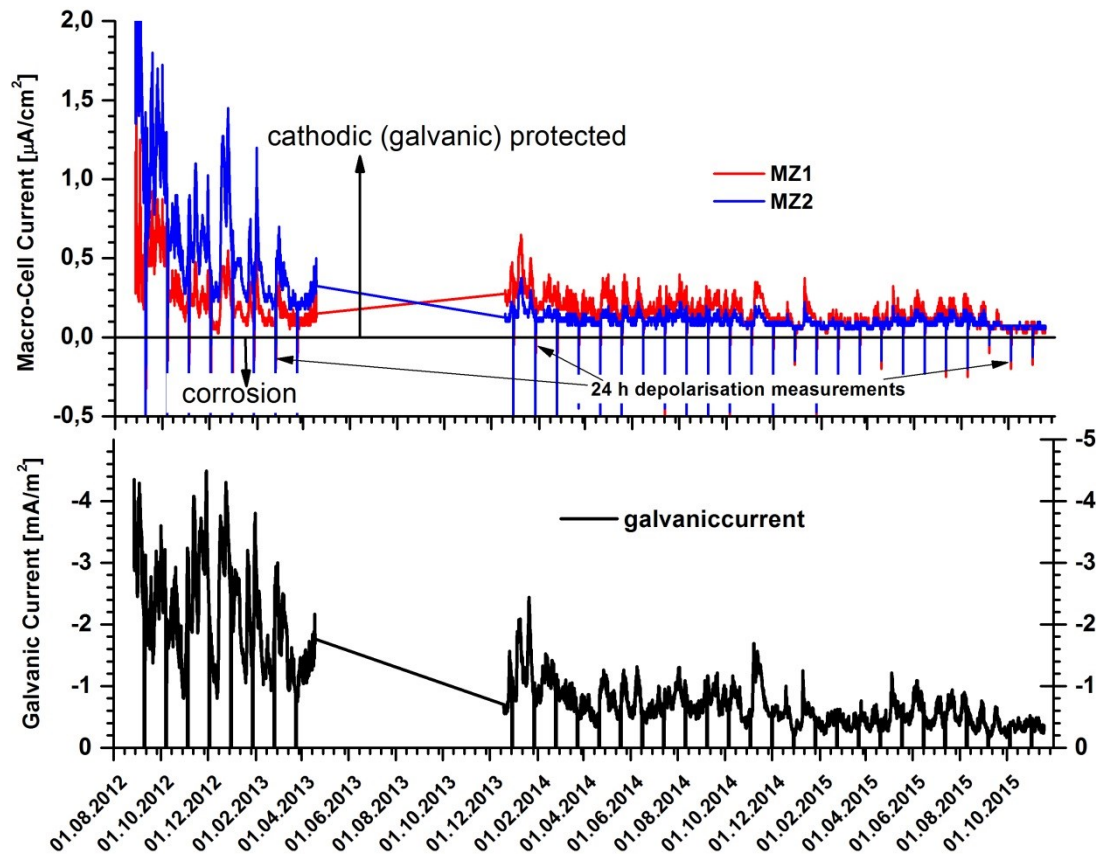
Figure 4. Galvanic Current of the EZA-System in relation to macro-cell currents measured by macro-cell sensors. Data from 1 August 2012 till 19 November 2015
