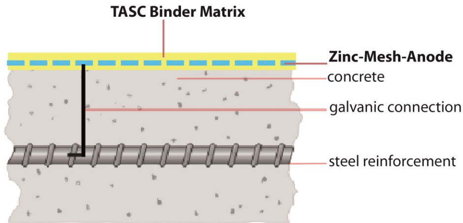
Figure 1. Embedded galvanic zinc anode (EZA): zinc mesh embedded into the EZA binder matrix
