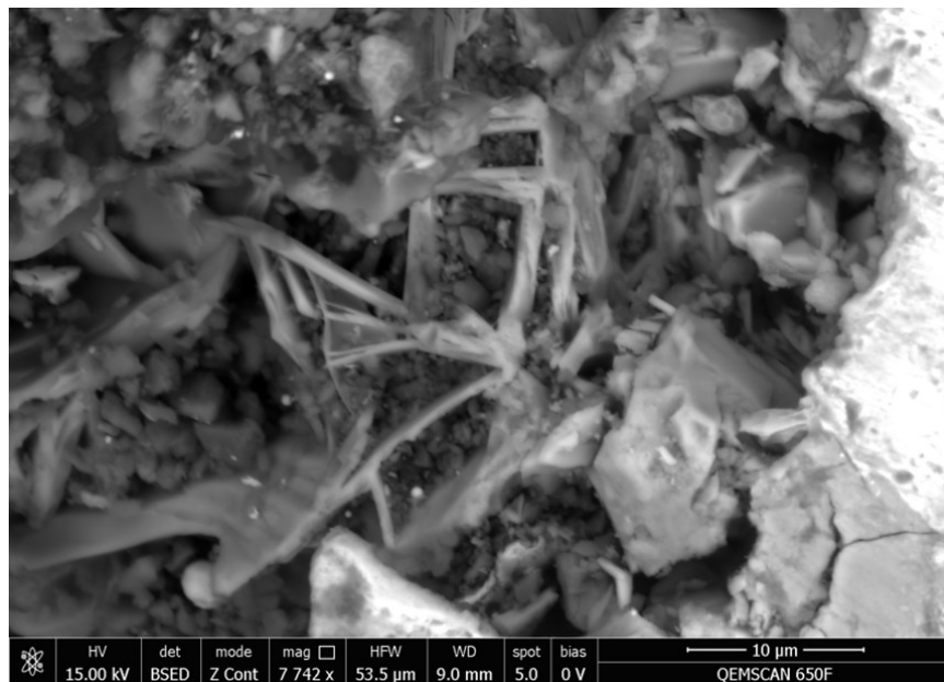
Figure 11. Zinc-hydroxychloride (Simonkolleite) precipitate near zinc anode
